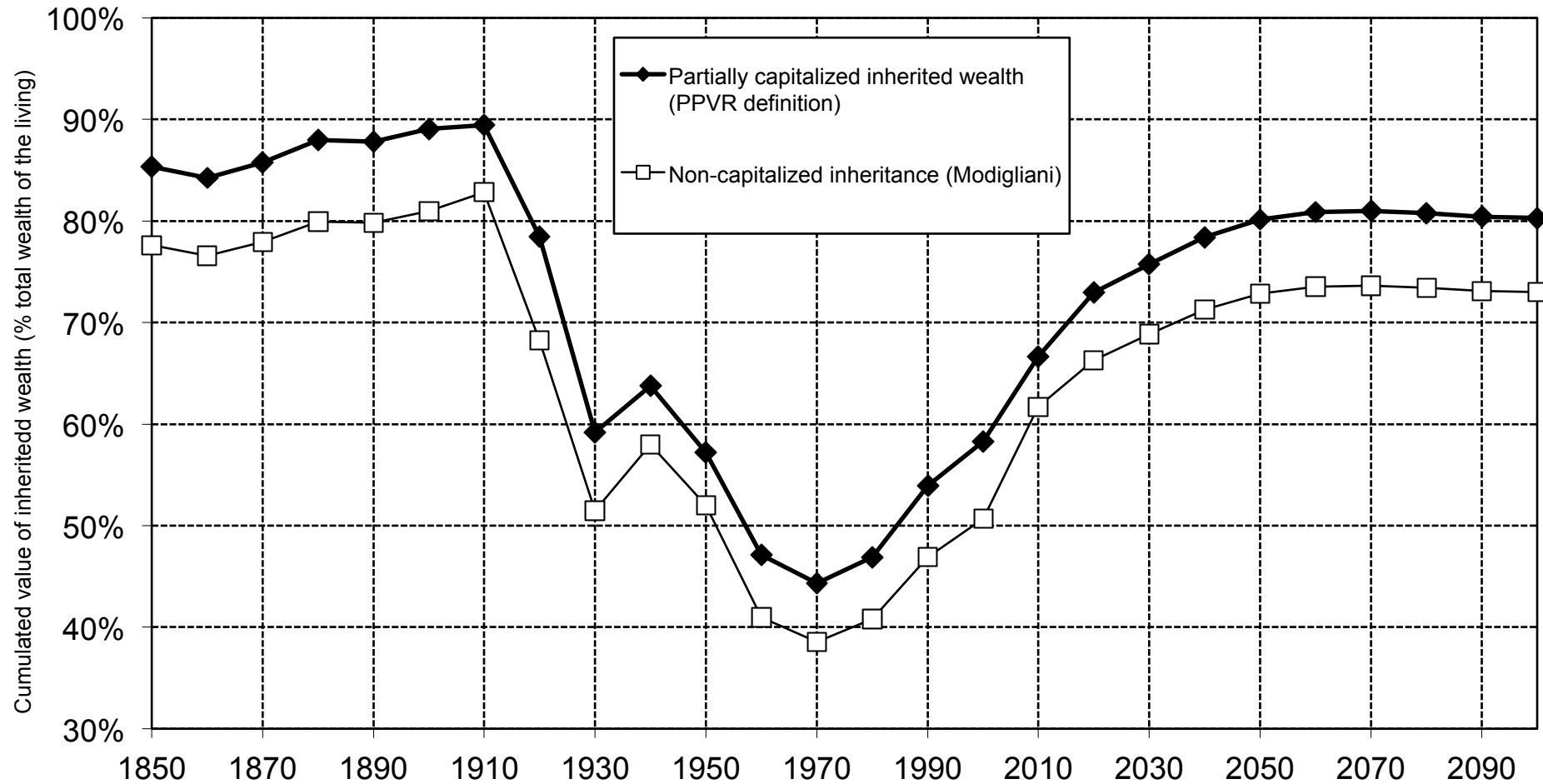
Figure S11.1. Share of inherited wealth in total wealth, France 1850-2100
