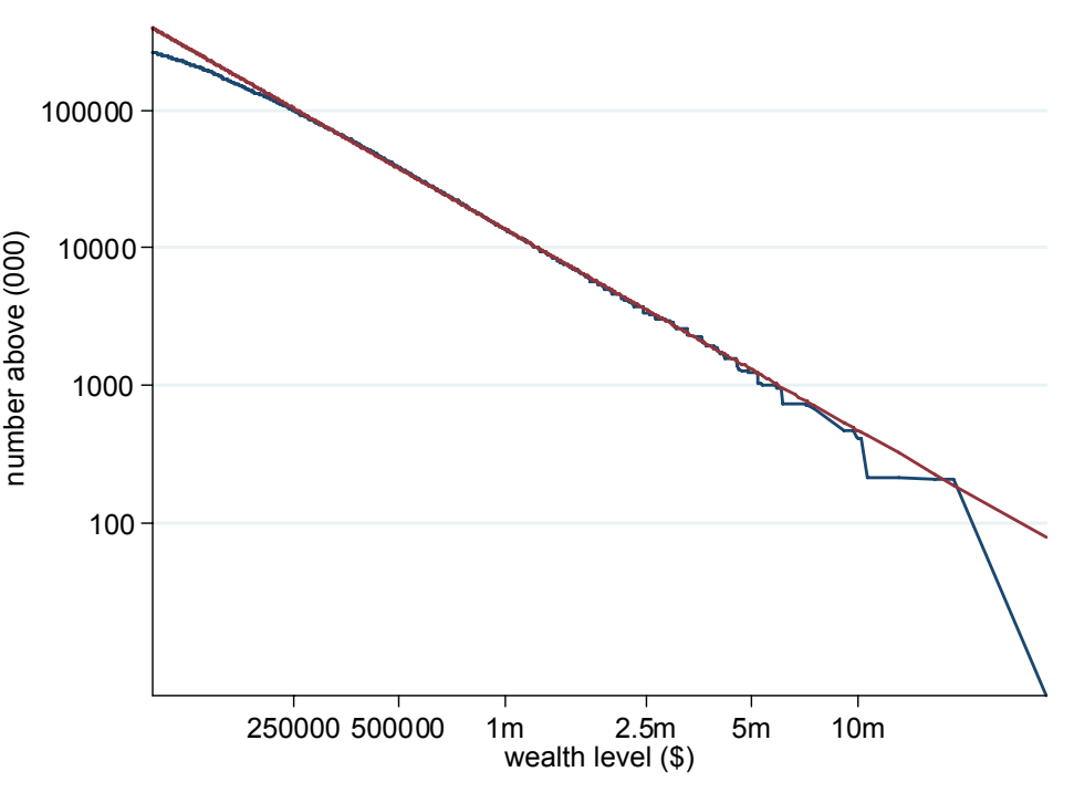
Figure 6: Fitted Parento distribution
